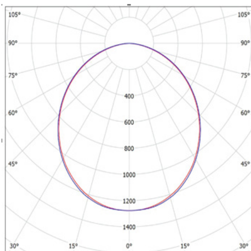
RHINO 45 RECESSED Polar Curve cd — C0-C180 — C90-C270
