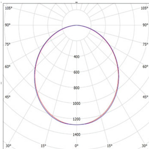
GREENSTAR 45 GS3 SQUARE Polar Curve cd — C0-C180 — C90-C270
